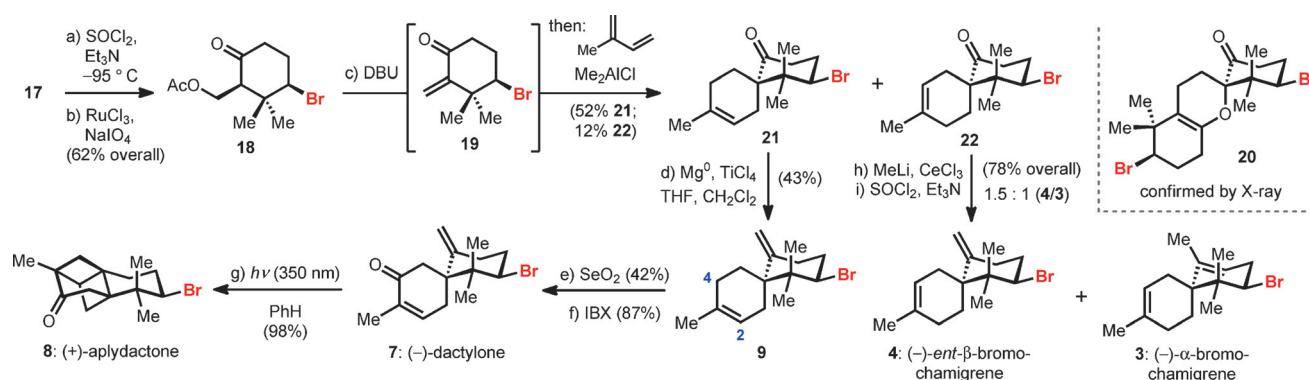
Scheme 3. Synthesis of (–)-dactylone, (+)-aplydactone, and (–)-α- and (–)-ent-β-bromochamigrene. Reagents and conditions: a) thionyl chloride (1.5 equiv), triethylamine (5 equiv), \text{CH}_2\text{Cl}_2 , -196 \rightarrow -95^\circ\text{C} ; b) ruthenium(III) chloride (0.02 equiv), sodium periodate (1.5 equiv), \text{MeCN}/\text{CCl}_4/\text{H}_2\text{O} , room temperature, 62 % from 17 ; c) 1,8-diazabicycloundec-7-ene (1.1 equiv), isoprene (20 equiv), \text{Me}_2\text{AlCl} (3.5 equiv), toluene, -78 \rightarrow -10^\circ\text{C} , 21 : 52%, 22 : 12%; d) magnesium (8.0 equiv), titanium tetrachloride (2.0 equiv), THF/ \text{CH}_2\text{Cl}_2 , 0^\circ\text{C} →RT, 43%; e) selenium dioxide (1.5 equiv), dioxane, 80^\circ\text{C} , 42%; f) 2-iodoxybenzoic acid (2.0 equiv), dimethyl sulfoxide, room temperature, 87%; g) h\nu (350 nm), benzene, room temperature, 98%; h) methyl lithium (4.5 equiv), cerium(III) chloride (5.0 equiv), THF, -78 \rightarrow 0^\circ\text{C} ; i) thionyl chloride (2.1 equiv), triethylamine (5.4 equiv), \text{CH}_2\text{Cl}_2 , -78 \rightarrow 0^\circ\text{C} , 78 % combined.
