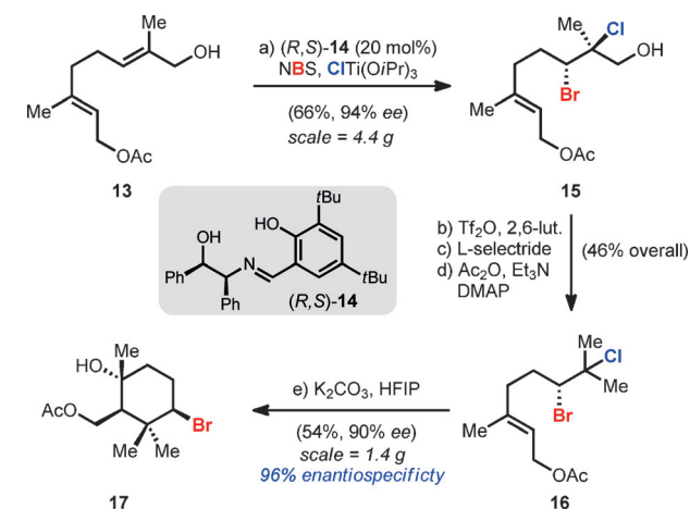
Scheme 2. Enantioselective dihalogenation and key solvolytic bromopolyene cyclization. Reagents and conditions: a) N -bromosuccinimide (1.05 equiv), \text{ClTi}(\text{OiPr})_3 (1.1 equiv), ( R,S )- 14 (20 mol %), hexanes, -20^\circ\text{C} , 66%; b) triflic anhydride (1.2 equiv), 2,6-lutidine (2.0 equiv), \text{CH}_2\text{Cl}_2 , -78^\circ\text{C} , 85%; c) L-selectride (5.5 equiv), THF, -78^\circ\text{C} →RT, 58%; d) acetic anhydride (1.0 equiv), 4-dimethylaminopyridine (0.05 equiv), triethylamine (1.2 equiv), \text{CH}_2\text{Cl}_2 , room temperature, 94%; e) potassium carbonate (1.5 equiv), hexafluoroisopropanol (0.05 M), room temperature, 54 %.
